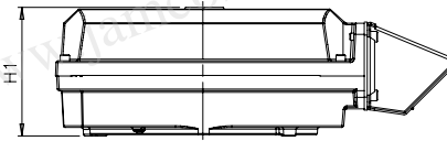
Motor sizes 355 - 400
