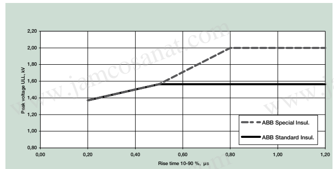
Figure 1. Allowed phase to phase voltage peaks at motor terminals as a function of rise time.
