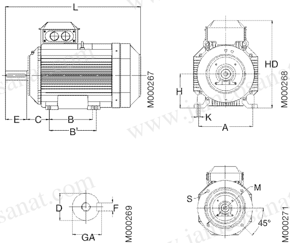
Sizes 71-200
