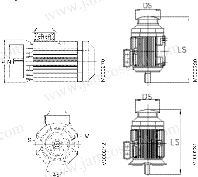
Sizes 225-400
