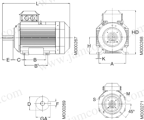
Sizes 71-200
