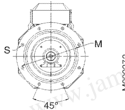
Sizes 225-400
