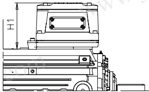
Motor sizes 280 - 315
