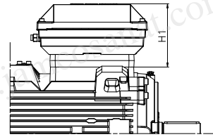
Motor sizes 200 - 250
