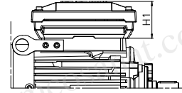
Motor sizes 80 - 132
