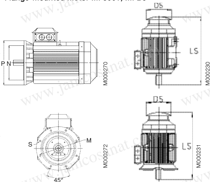
Sizes 225-355
